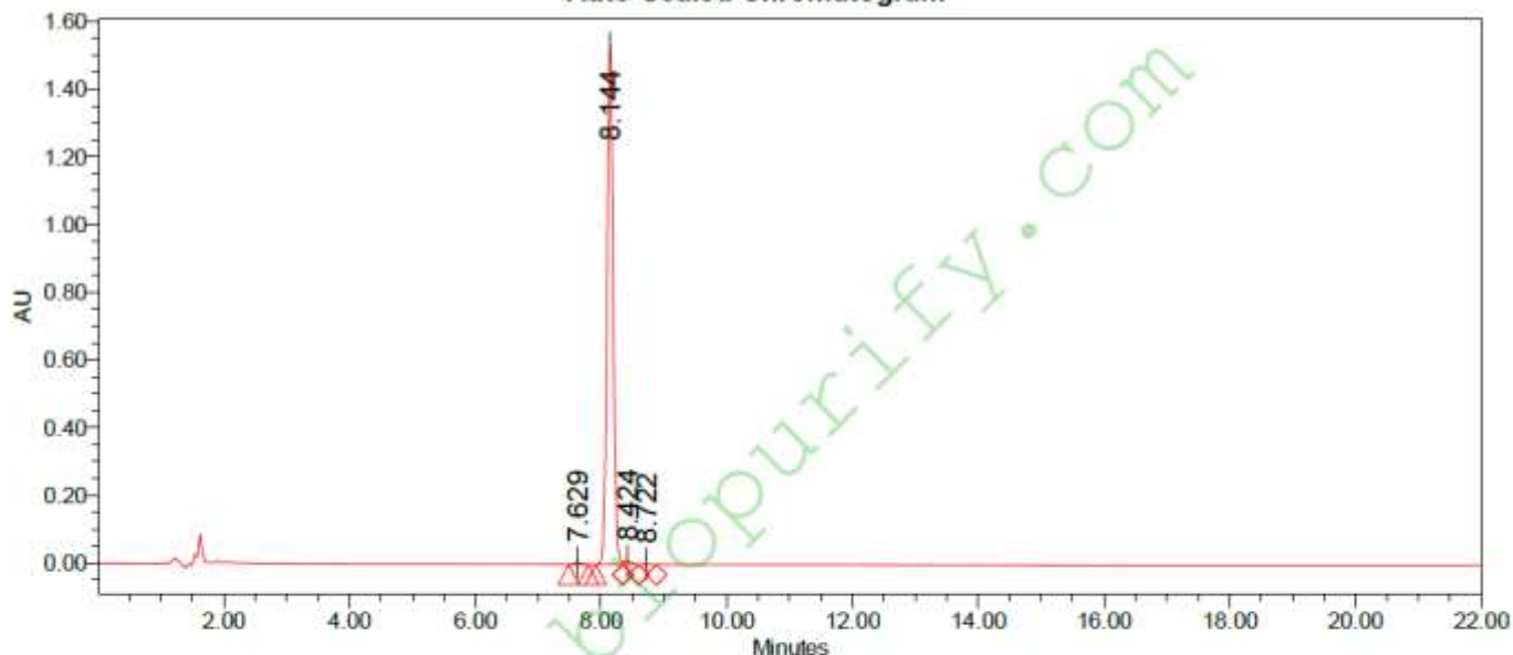
Auto-Scaled Chromatogram
